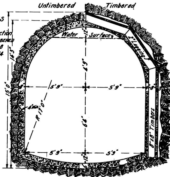
TUNNEL SECTIONS SOUTH OF FAIRMONT RESERVOIR
